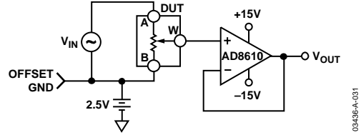
Figure 32. Test Circuit for Gain vs. Frequency
