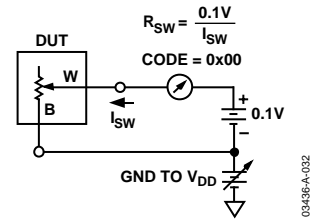
Figure 33. Test Circuit for Incremental ON Resistance
